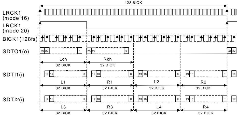
Figure 9. Mode 16 ,20 Timing
