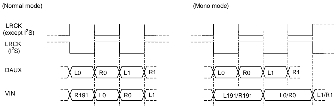
Figure 22. DAUX2 and VIN input timings
