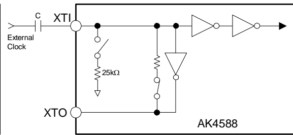
Figure 19. (b). External clock mode (Input : ≥40% DVDD)
