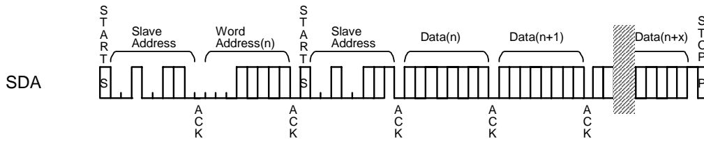
Figure 49. RANDOM READ
