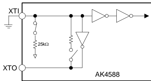
Figure 20. OFF mode
